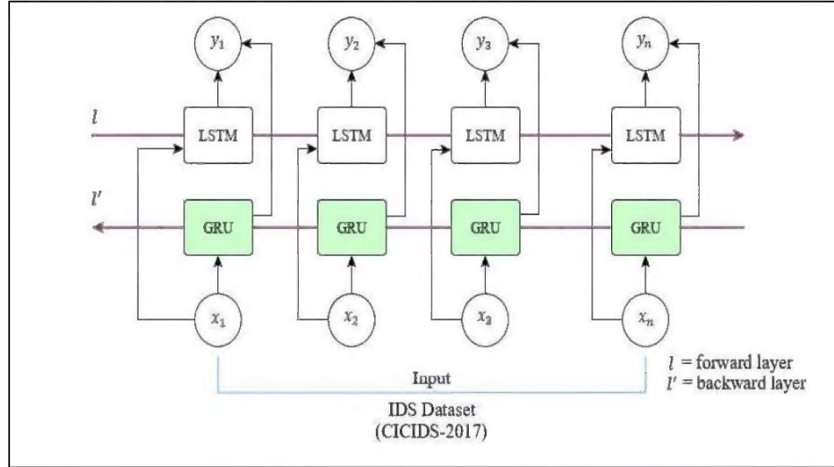
Figure 2. Bidirectional RNN Architecture
