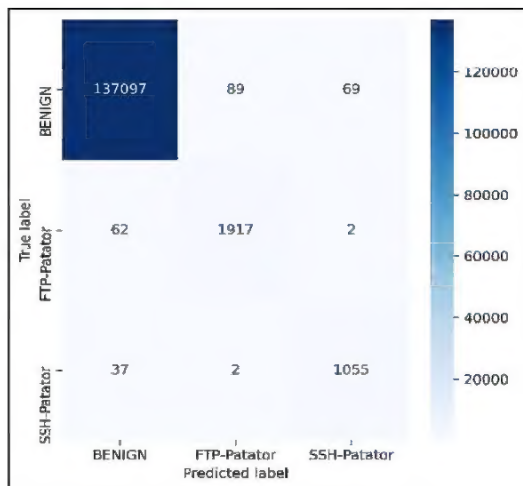
Figure 3: Tuesday: Confusion Matrix data set
