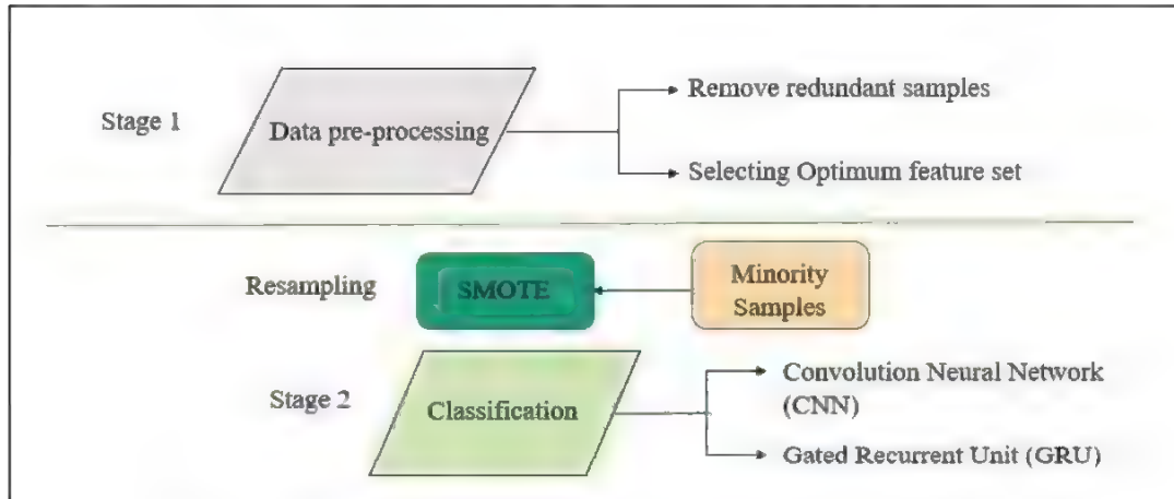
Figure 7: Proposed Model. SMOTE: Synthetic Minority Oversampling Technique
