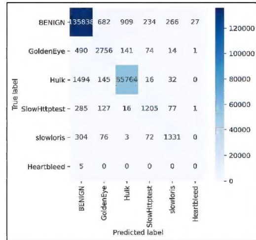
Figure 4: Wednesday Confusion Matrix data set
