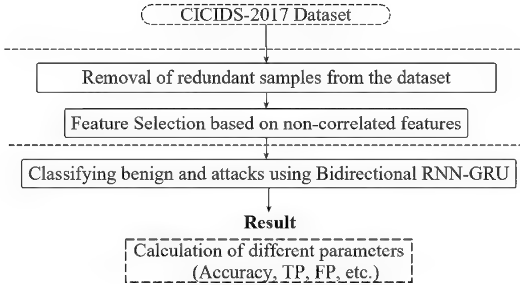
Figure 6. Proposed Model Layout
