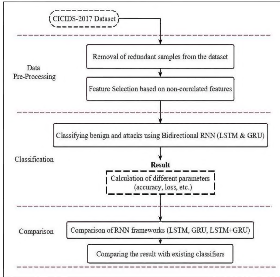
Figure 1: Proposed Model layout
