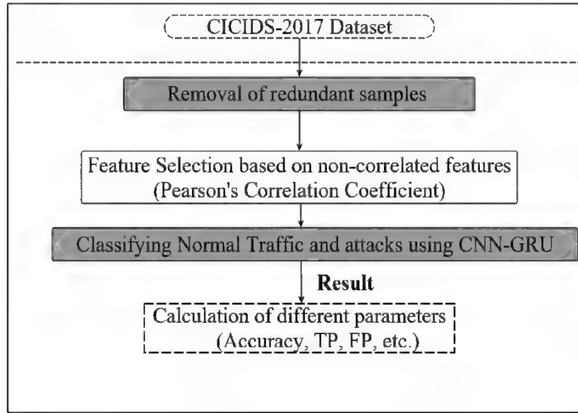
Figure 5. Proposed Model Layout
